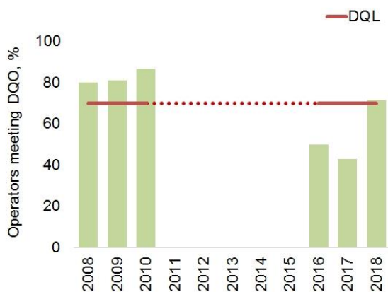
Figure 6-2. Frequency of operators that met the DQO of \geq 70\% in scoring symptoms induced or not by ozone, in photo exercises carried out during the more recent UNECE-ICP Forests Intercalibration courses on the assessment of ozone visible symptoms.
