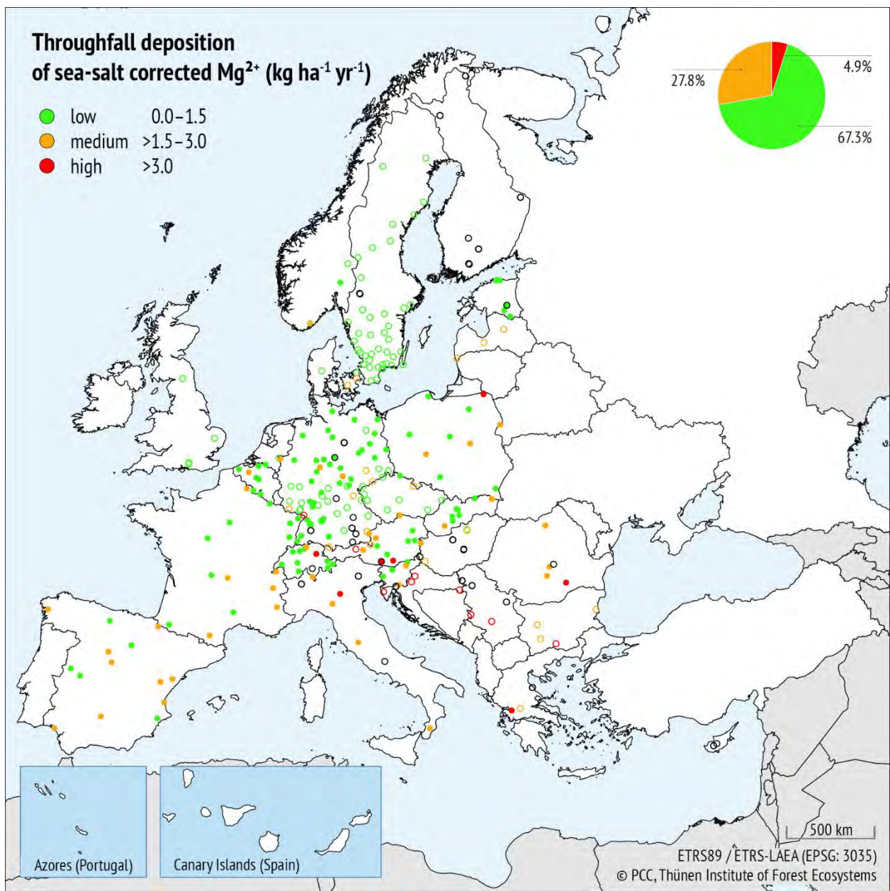
Figure 5-7: Throughfall deposition of sea-salt corrected magnesium ( kg\ Mg^{2+}\ ha^{-1}\ yr^{-1} ) measured in 2021 on the ICP Forests Level II plots and the Swedish Throughfall Monitoring Network. Colored dots: validated data. Colored circles: not validated data. Black circles: monitoring period shorter than 330 days or irregular sampling.
