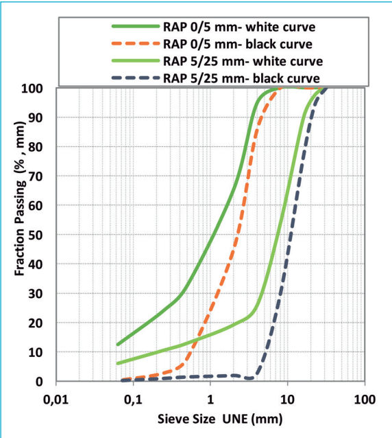
Figure 1 . RAP original gradations and after extraction aged binder
